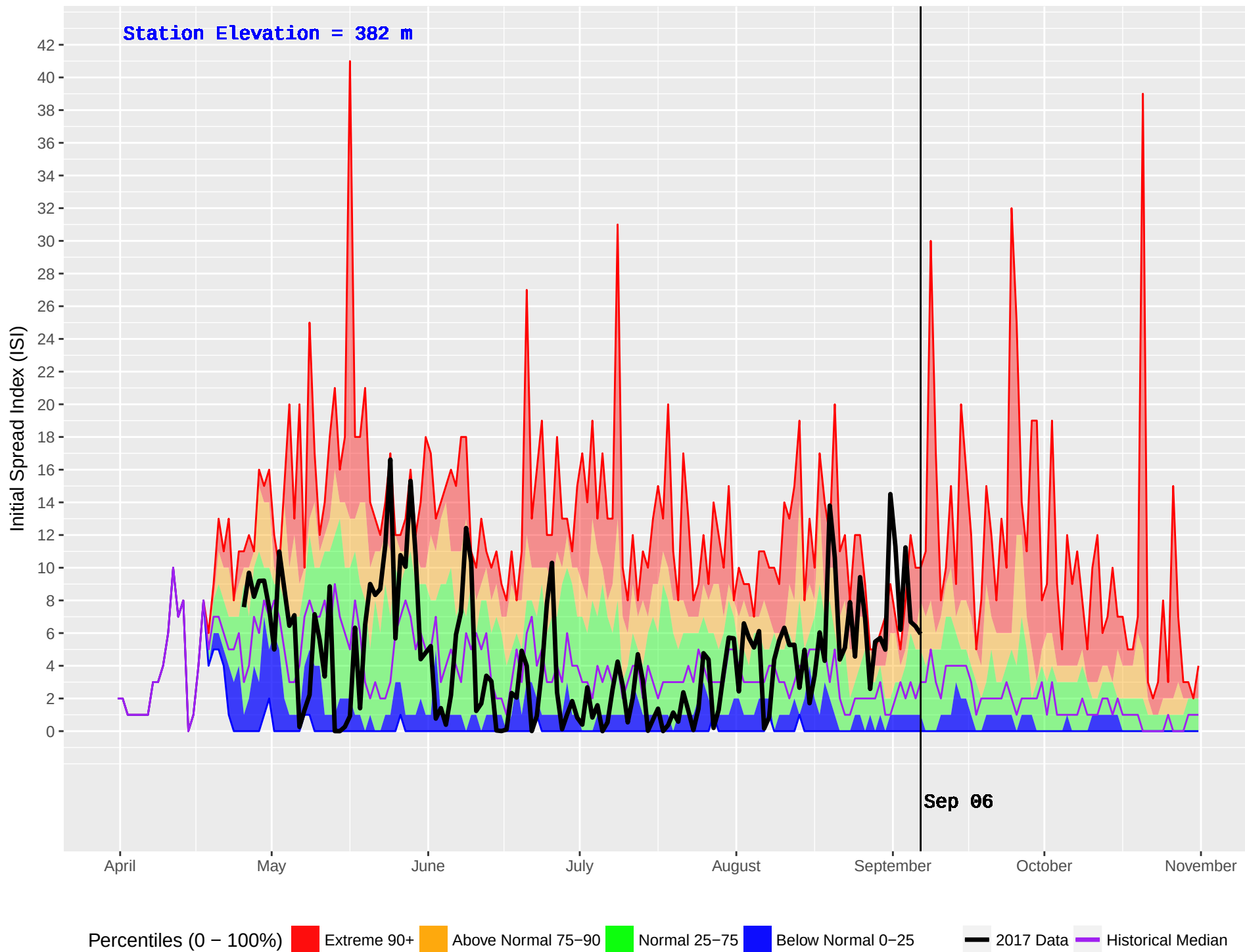
FORT NELSON FS (599) : Historical (1999–2016) and Current (2017) Noon Initial Spread Index (ISI)
