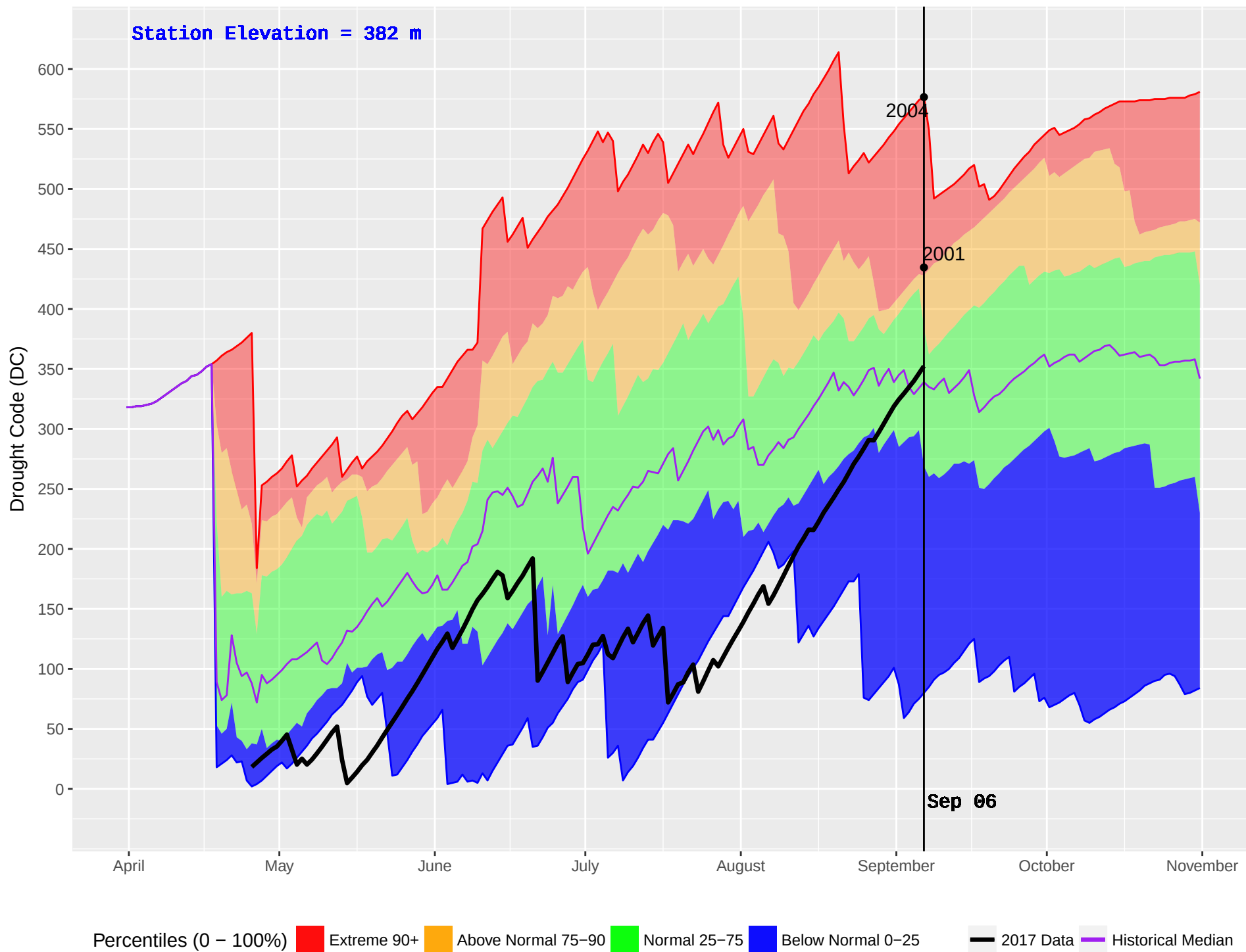
FORT NELSON FS (599) : Historical (1999–2016) and Current (2017) Noon Drought Code (DC)
